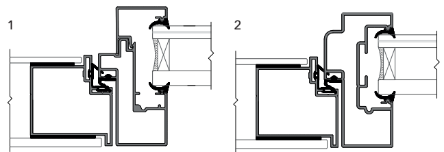
DEKO FG SILENT - FULLY GLAZED PARTITION
