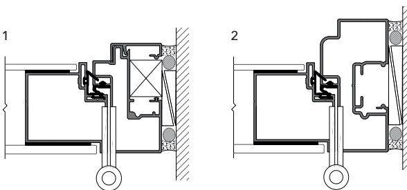
GYPSUM WALL
