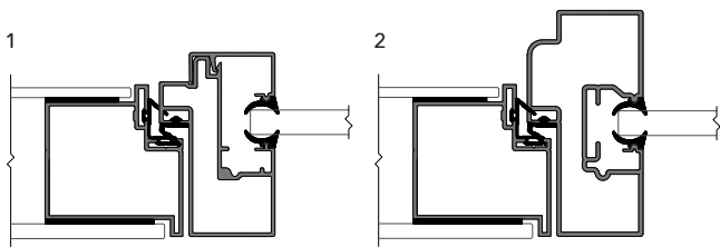
DEKO FG - FULLY GLAZED PARTITION
