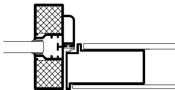
DEKO FG fully glazed partition
