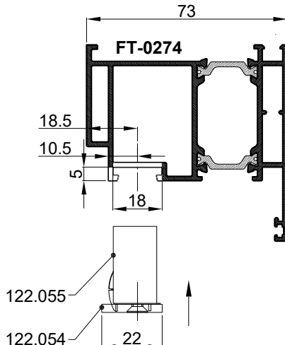
PRESJEK 2-2 CROSS SECTION 2-2
