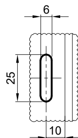
POGLED 2-2 VIEW 2-2
