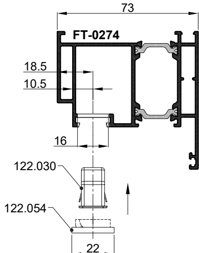
PRESJEK 1-1 CROSS SECTION 1-1
