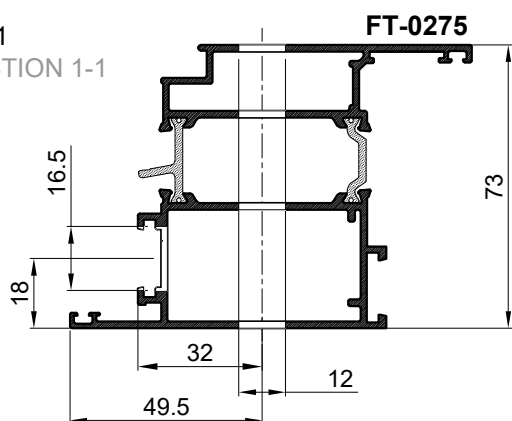
PRESJEK 2-2 CROSS-SECTION 2-2
