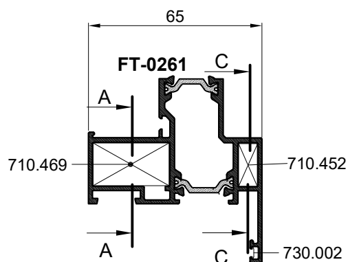
PRESJEK B-B CROSS-SECTION B-B
