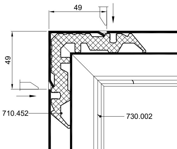
PRESJEK C-C CROSS-SECTION C-C
