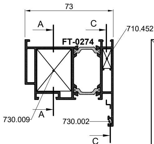
PRESJEK B-B CROSS-SECTION B-B
