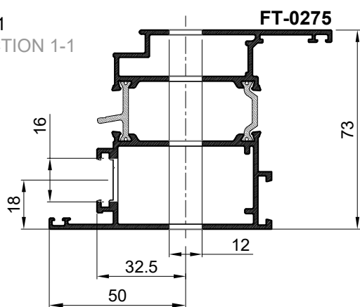
PRESJEK 2-2 CROSS-SECTION 2-2
