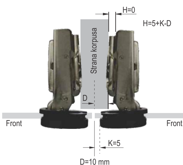
Polukoleno (B)
