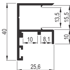
Al gornji profil (1,5m; 2m; 3m; 4m i 6m)
