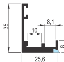
Al donji profil (1,5m; 2m; 3m; 4m i 6m)
