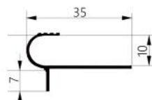
ST 350 UC step. al. profil
