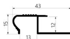
ST 390 step. al. profil
