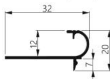
ST 355 UC step. al. profil
