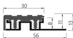
ST 380 step. al. profil
