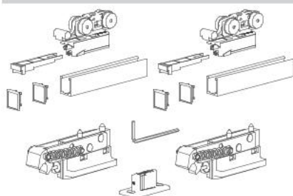
PVD TS-EVOLUTION/40 meh.-usp.
