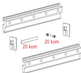
PVD V40 nosač stakla 8mm TS
