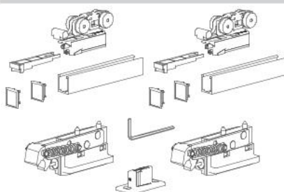
PVD TS-EVOLUTION/60 meh.-usp.
