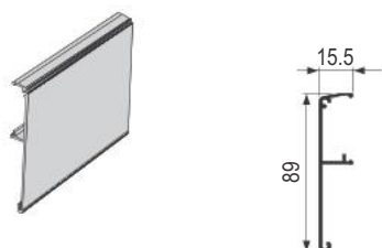
PVD TS-1700/1280 maska AL (PVS)
