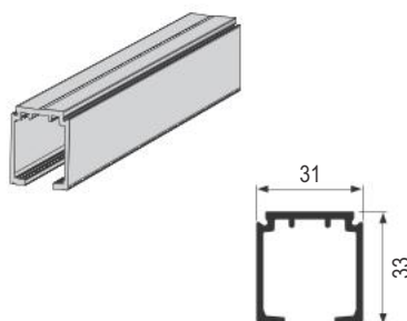
PVD TS-1280 gornja šina AL (PVS)
