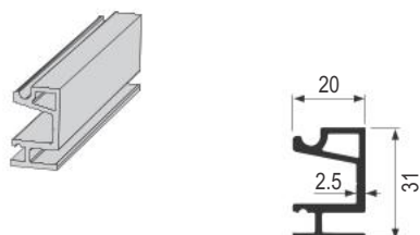
PVD TS-1700 nosač 1710 AL(PVS)
