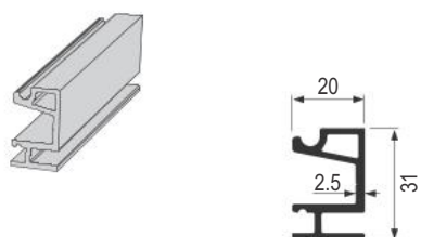
PVD TS-1700 nosač 1710 AL(PVS)
