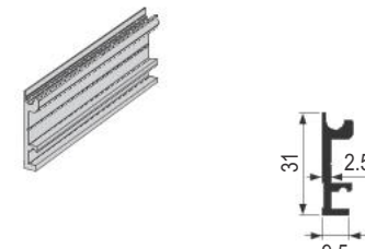
PVD TS-1700 nosač 1720 AL(PVS)
