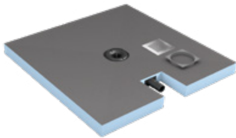
E.g. Fundo Plano 65 mm thick flush-to-floor shower element with integrated point drainage
